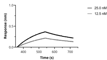
BLI binding kinetics of SARS-CoV-2 Spike Recombinant VHH [NM1222] to RBD. Biotinylated RBD was immobilized on FortéBio Streptavidin (SA) Biosensors and assayed with different concentrations of SARS-CoV-2 Spike Recombinant VHH [NM1222] (ChromoTek sc-NM1222).
