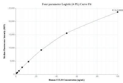
Cytometric bead array standard curve of MP01301-2, CCL20/MIP-3 alpha Recombinant Matched Antibody Pair, PBS Only. Capture antibody: 84413-1-PBS. Detection antibody: 84413-2-PBS. Standard: Eg2398. Range: 0.781-100 ng/mL
