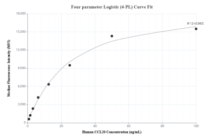
Cytometric bead array standard curve of MP01301-3, CCL20/MIP-3 alpha Recombinant Matched Antibody Pair, PBS Only. Capture antibody: 84413-3-PBS. Detection antibody: 84413-2-PBS. Standard: Eg2398. Range: 0.781-100 ng/mL
