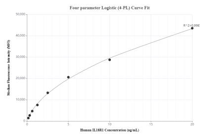
Cytometric bead array standard curve of MP01261-3, IL18R1 Recombinant Matched Antibody Pair, PBS Only. Capture antibody: 84390-3-PBS. Detection antibody: 84390-1-PBS. Standard: RP00006. Range: 0.156-20 ng/mL
