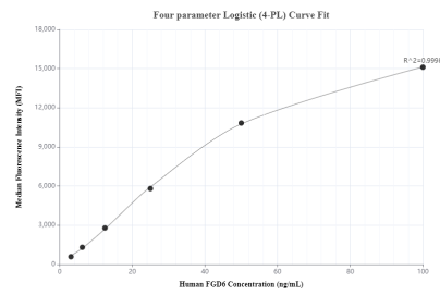
Cytometric bead array standard curve of MP00314-2, FGD6 Recombinant Matched Antibody Pair, PBS Only. Capture antibody: 83296-2-PBS. Detection antibody: 83296-1-PBS. Standard: Ag22211. Range: 3.13-100 ng/mL
