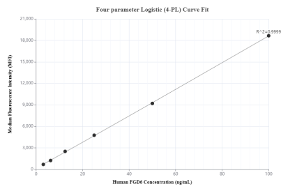
Cytometric bead array standard curve of MP00314-1, FGD6 Recombinant Matched Antibody Pair, PBS Only. Capture antibody: 83296-3-PBS. Detection antibody: 83296-1-PBS. Standard: Ag22211. Range: 3.13-100 ng/mL
